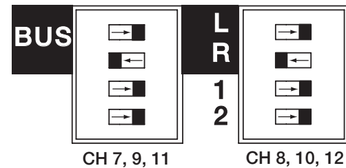
BUS DIP Switch Settings (CH 7-12)
