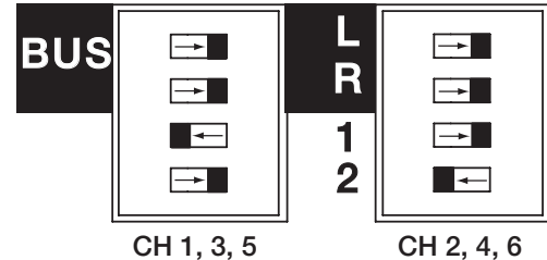
BUS DIP Switch Settings (CH 1-6-Factory Default)
